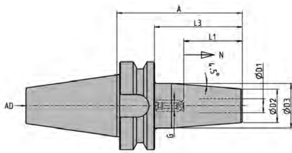
T... JD 50 (Alt/Old: BT50, MAS403)
