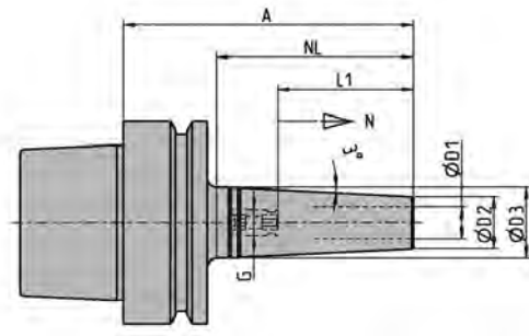
TSF... HSK-E50 – Inch
