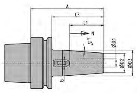
T... HSK - E50 – Inch
